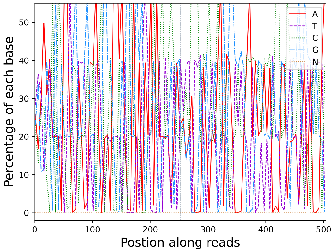
Base percentage along reads (R10309)
